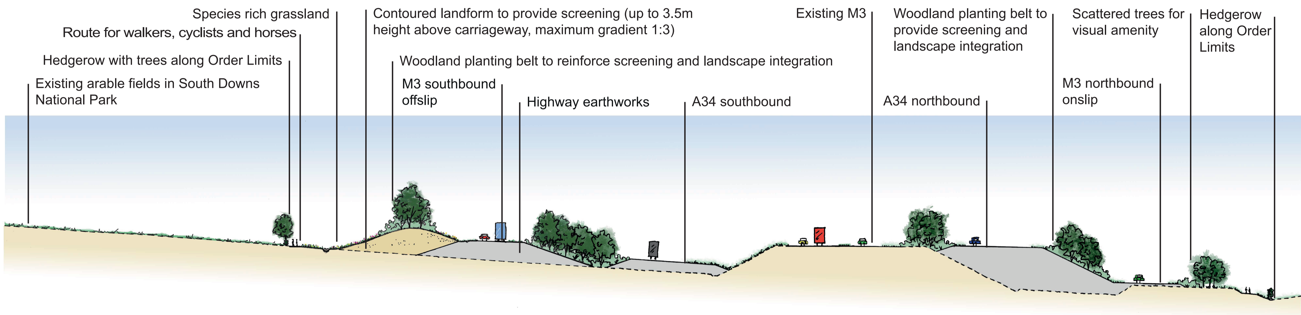
TYPICAL CROSS SECTION 2 Approximate chainage: 520
