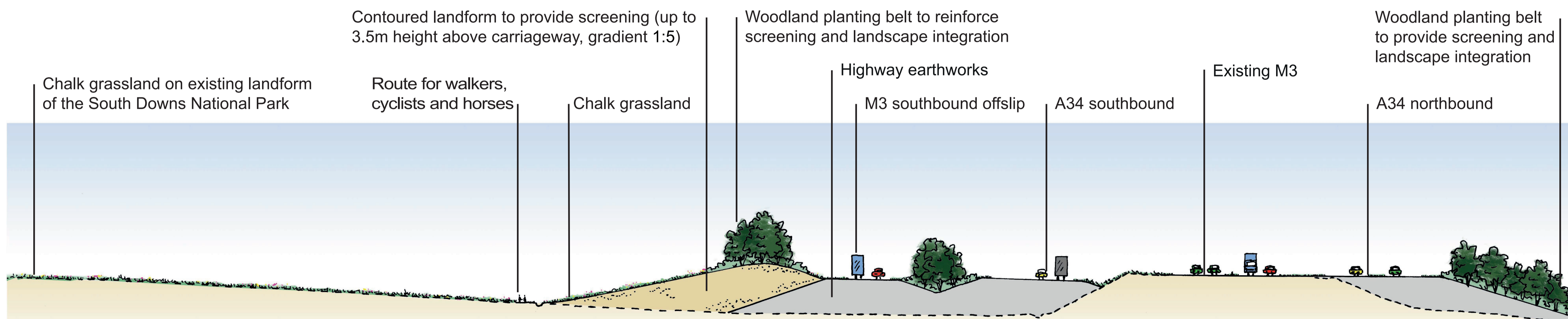
TYPICAL CROSS SECTION 3 Approximate chainage: 620
