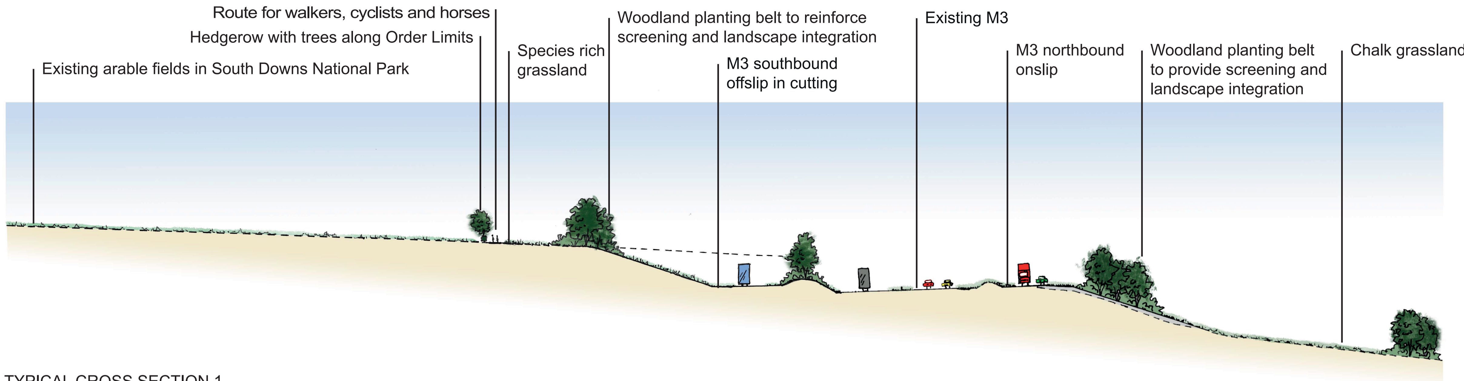
TYPICAL CROSS SECTION 1 Approximate chainage: 160
