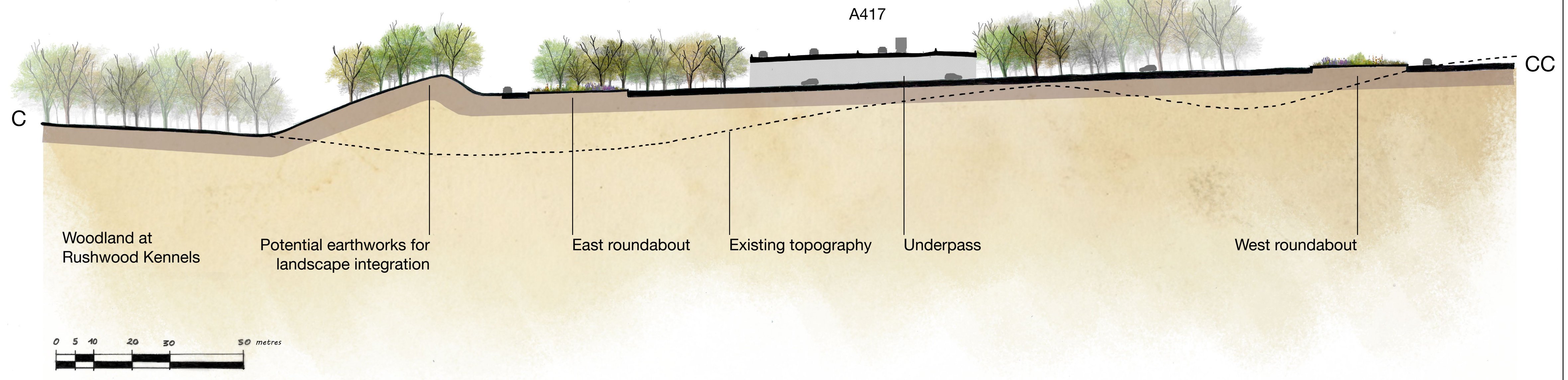
INDICATIVE CROSS SECTION AT SHAB HILL
