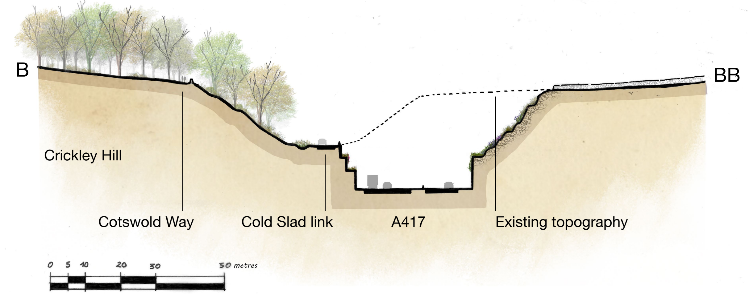
INDICATIVE CROSS SECTION AT CRICKLEY HILL
