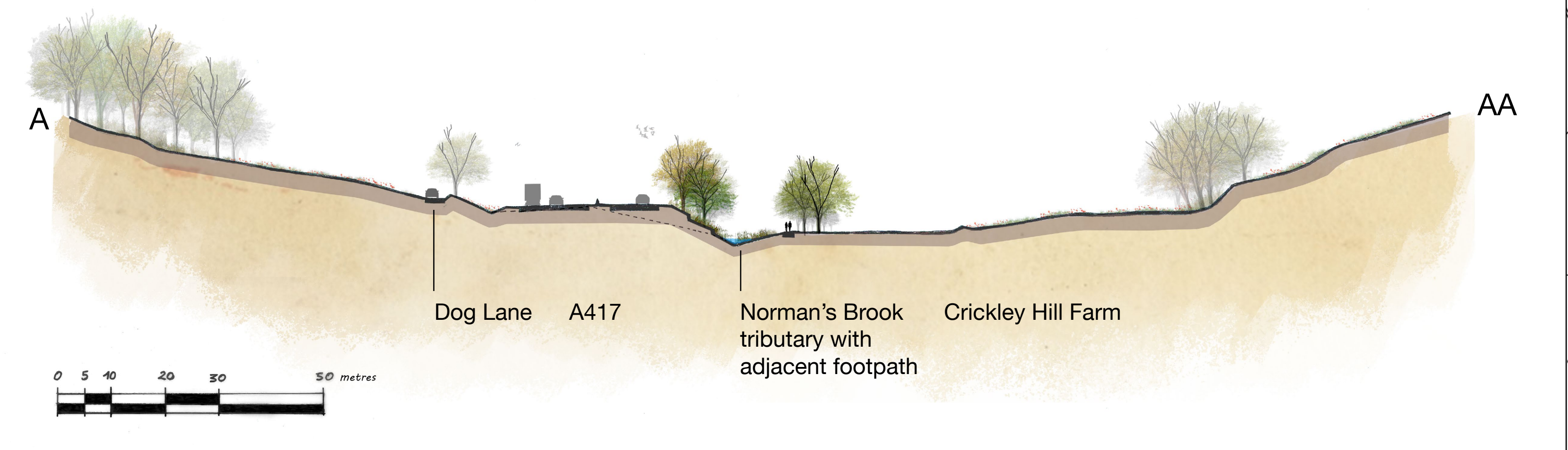
INDICATIVE CROSS SECTION AT DOG LANE AND CRICKLEY HILL FARM
